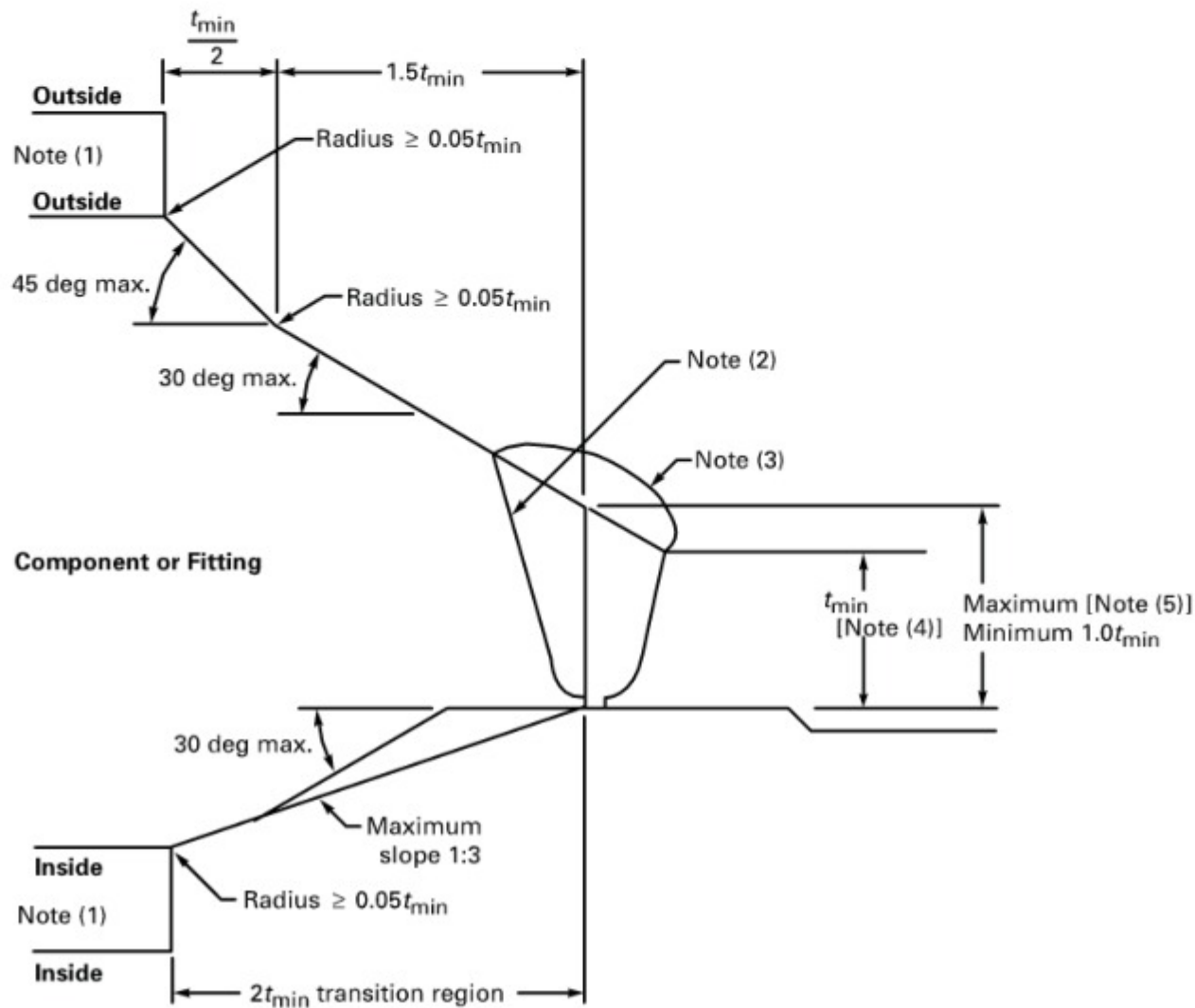
Figure 1 Maximum Envelope for Welding End Transitions
